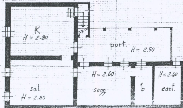
PIANO TERRA
